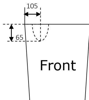
Cistern Front View The back inlet locates on the top left corner when you face the water tank
